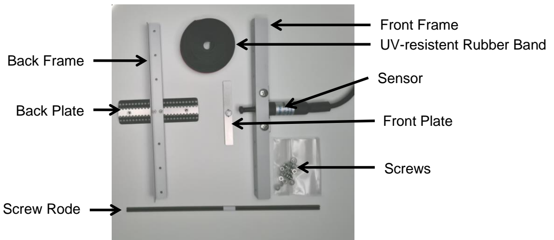
Waterproof Diameter Dendrometer
